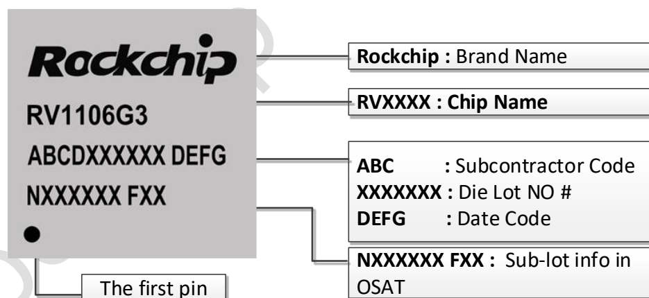
Fig.2-2 RV1106G3 Package definition
